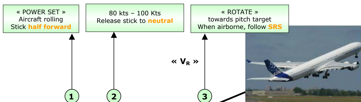
Figure 2 Typical Takeoff Sequence
